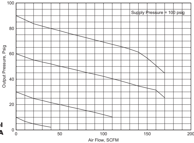
Flow Characteristics Fairchild Model 2564A
